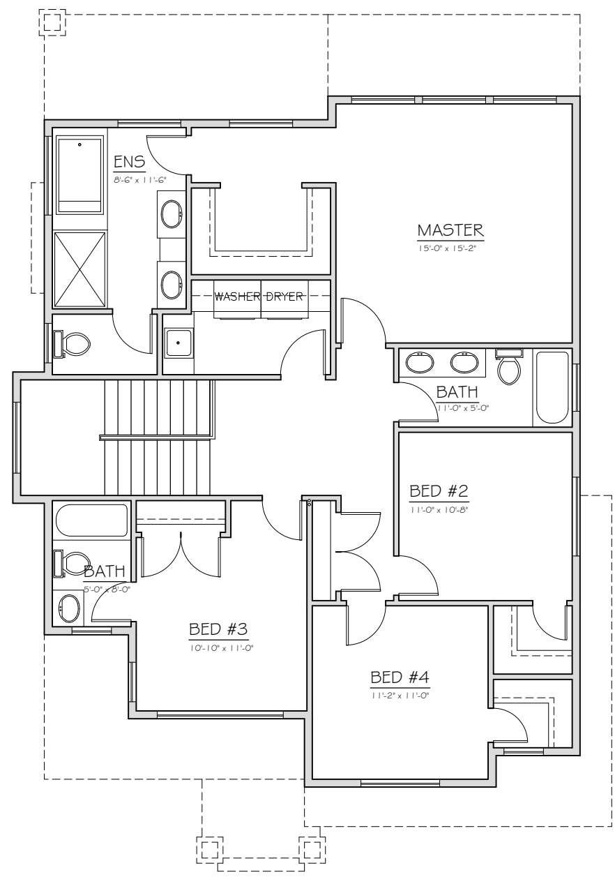
UPPER FLOOR LIVING - 1,281.00 sq. ft. STAIRS - 92.00 sq. ft. TOTAL - 1,373.00 sq. ft.
