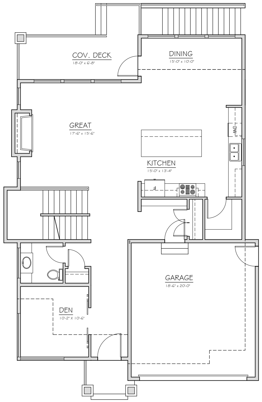
MAIN FLOOR LIVING - 1,230 sq. ft. GARAGE - 410 sq. ft. TOTAL - 1,640 sq. ft.
