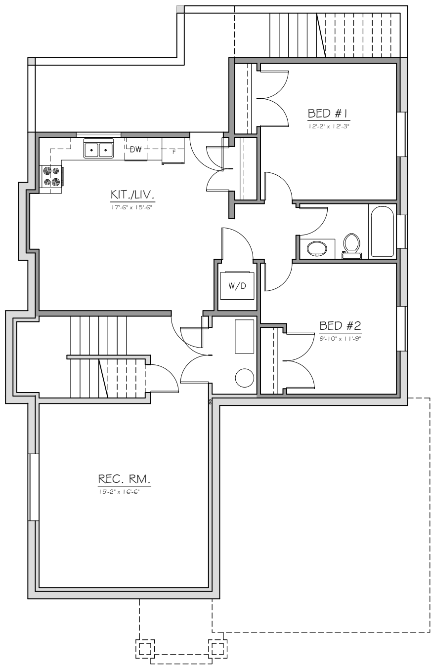
BASEMENT FLOOR LIVING - 460.00 sq. ft. SUITE - 776.00 sq. ft. TOTAL - 1,236.00 sq. ft.
