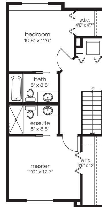
SECOND LEVEL +/- 593 sq. ft.
