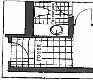
LAYOUT FOR SUITE 3 (29 TO 44th FLOOR)
