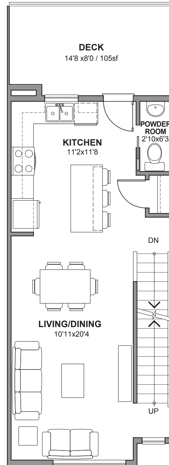
MAIN FLOOR PLAN - UNIT 'B'
