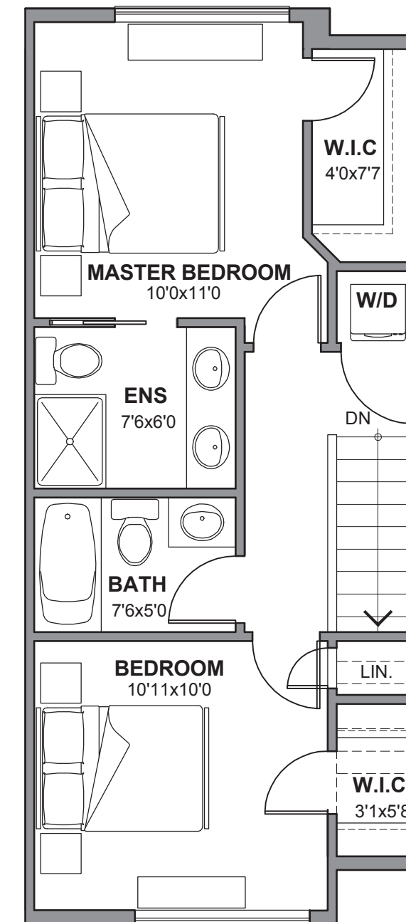
UPPER FLOOR PLAN - UNIT 'B'
