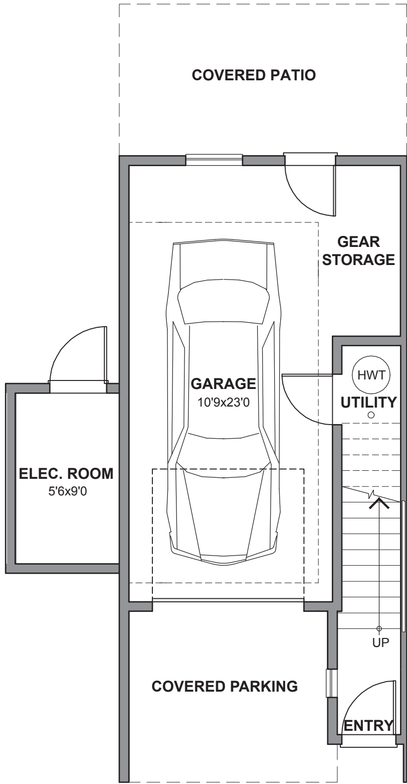
LOWER FLOOR PLAN - UNIT 'B2'
