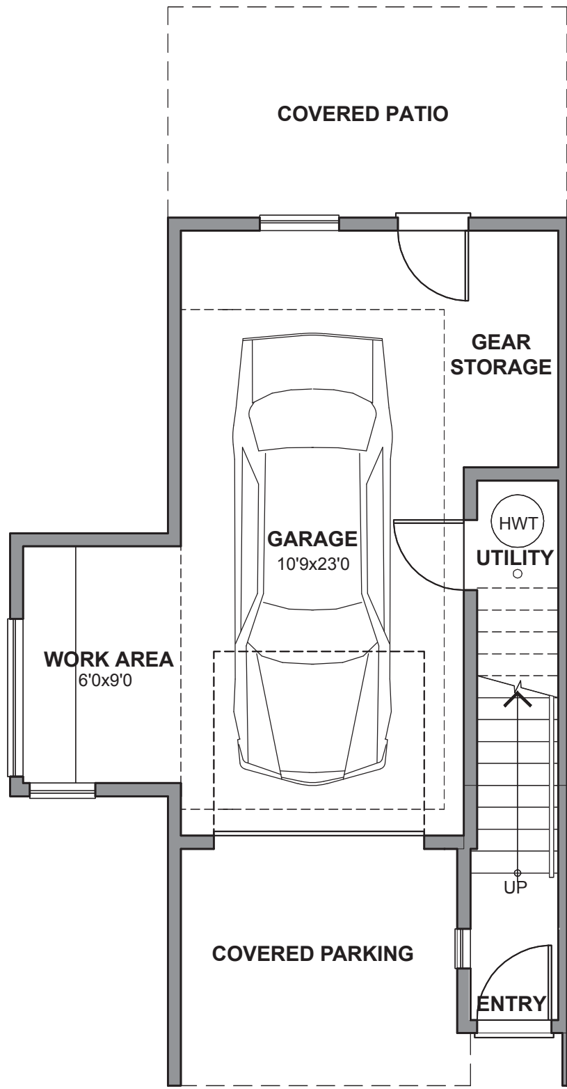
LOWER FLOOR PLAN - UNIT 'B1'
