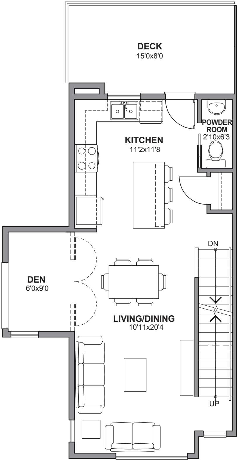
MAIN FLOOR PLAN - UNIT 'B1'
