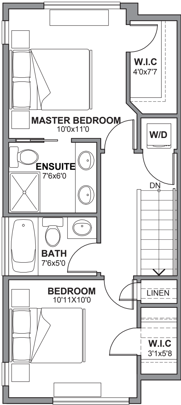
UPPER FLOOR PLAN - UNIT 'B1'
