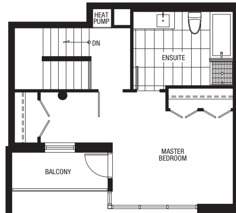
3ND FLOOR
