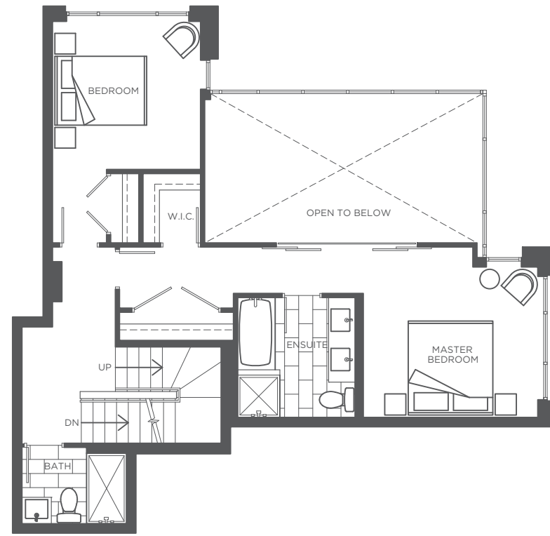
UPPER FLOOR 715 sq ft (approx)
