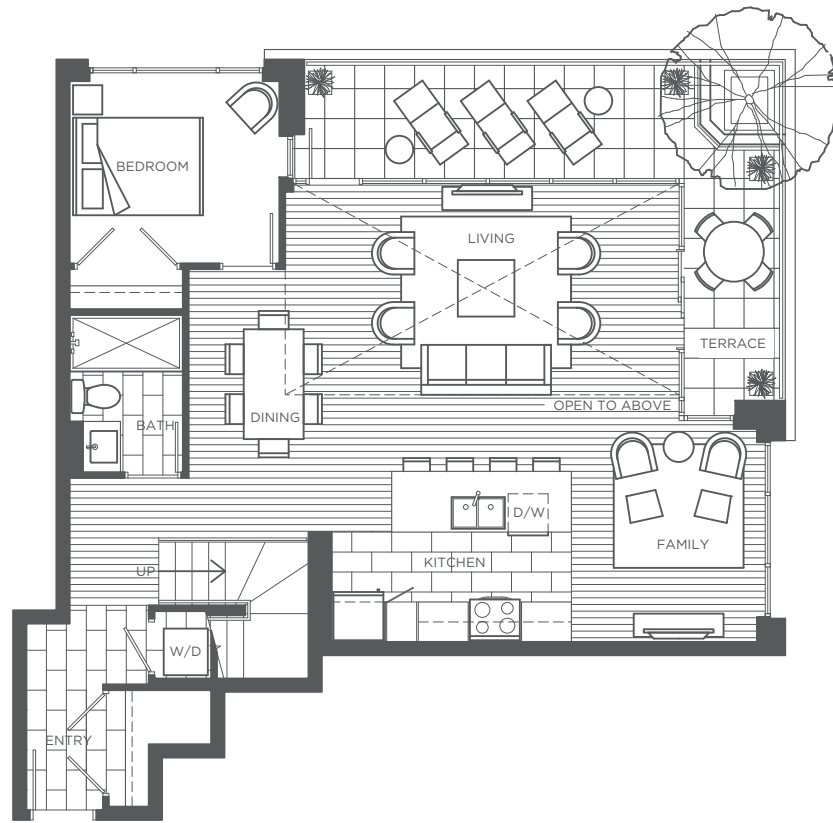
LOWER FLOOR 930 sq ft (approx) TERRACE 185 sq ft (approx)
