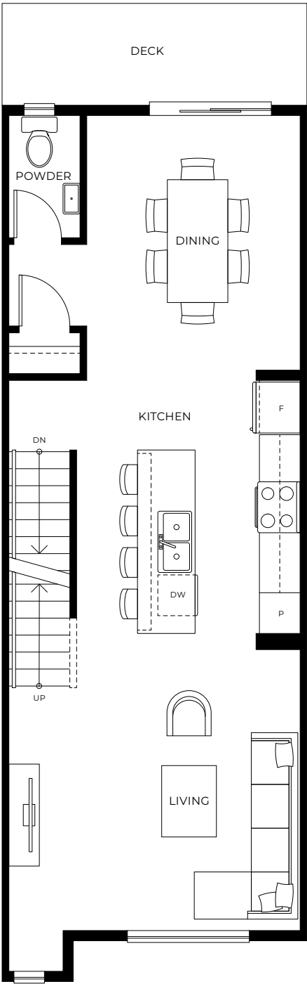
Main Floor
