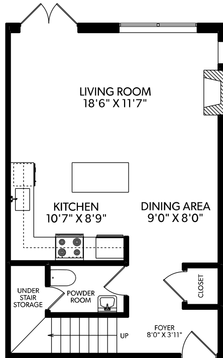
MAIN FLOOR
