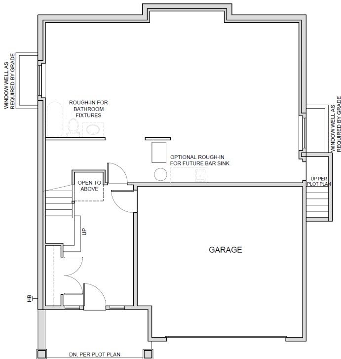
UNFINISHED BASEMENT
