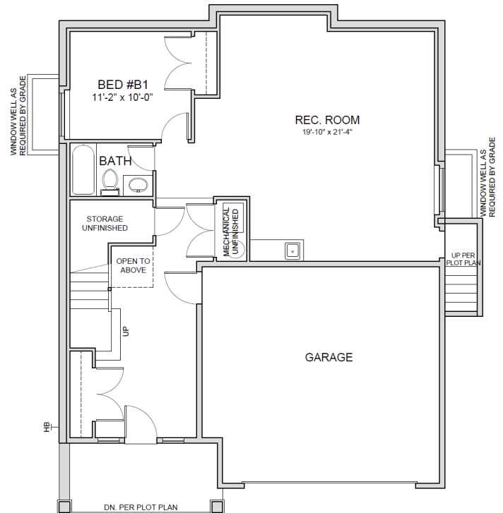
FINISHED BASEMENT
