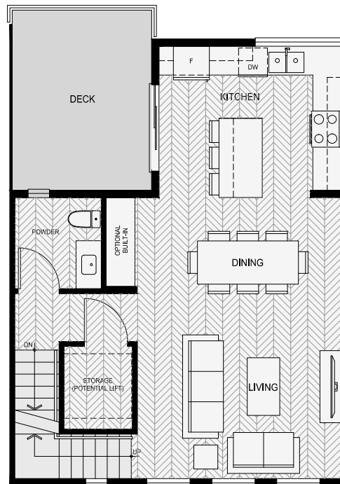
MAIN FLOOR
