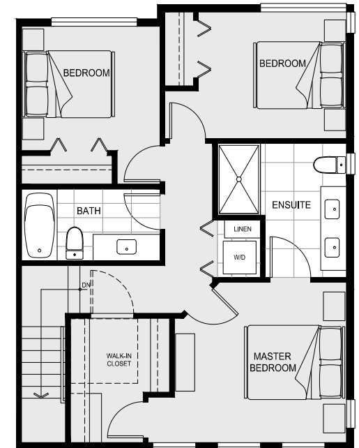
UPPER FLOOR
